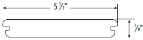
5/4 x 6 Channeled™
